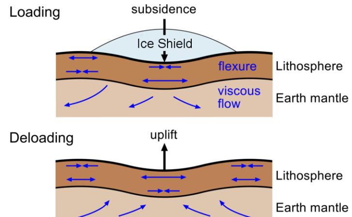
Abb. 5: Glacial Isostatic Adjustment. Grafik aus [4].
